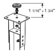
With leg extensions WS21
