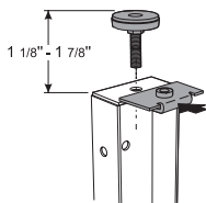
For leg WS20/25
