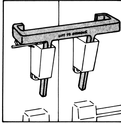
MODEL SL-410 OR SL-415* DOUBLE DOOR LATCH For doors without a center post.
